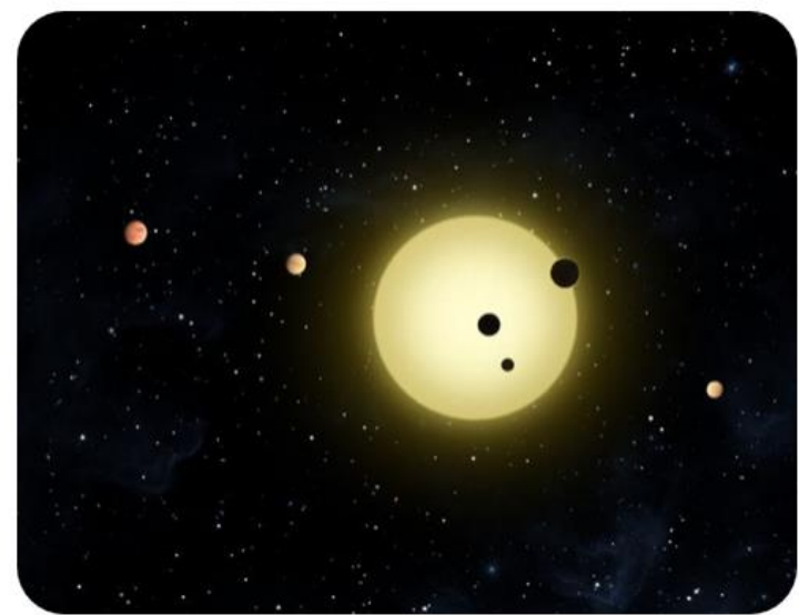
An artist's representation of Kepler-11, a small, cool star around which six planets orbit. Credit: NASA/Tim Pyle
