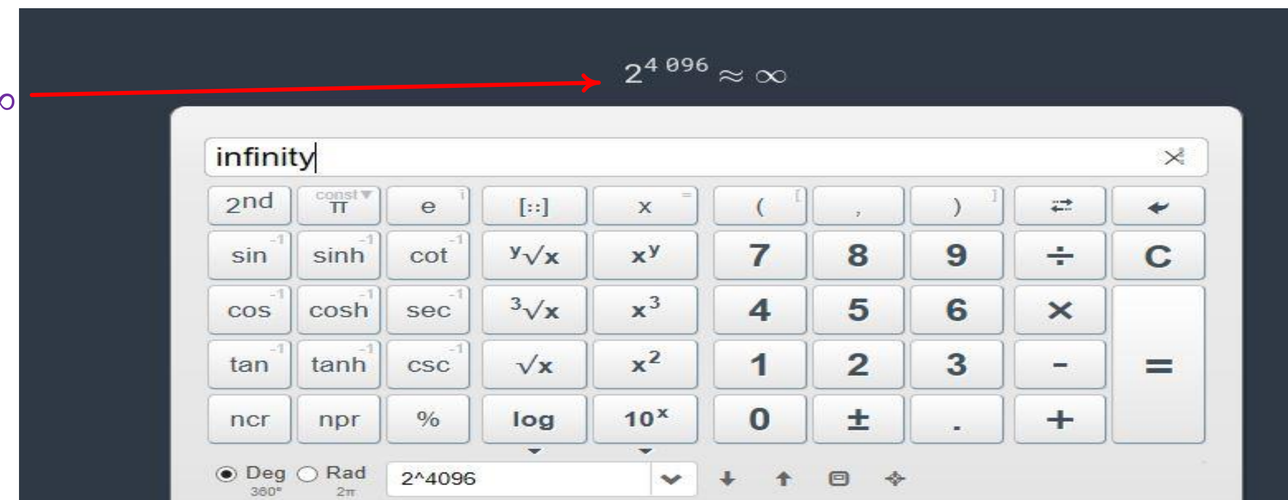
Power of 2 by 10 levels of 2^4096
